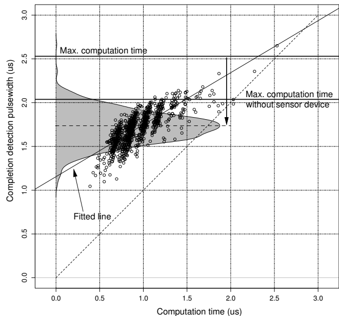
Fig. 9. Comparison of the actual computation time of the 16-bit adder and the monostable multivibrator response for randomly generated input vectors, showing the time-domain gain obtained by the proposed approach.
