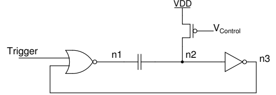
Fig. 7. Basic monostable multivibrator with variable resistor.
